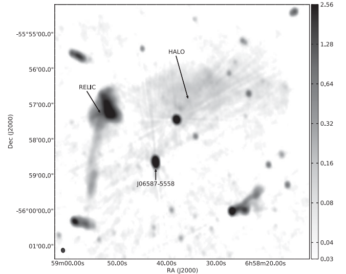
Figure 2. A primary beam corrected, medium-resolution (synthesized beam FWHM \approx 7 arcsec), Stokes I , 1.1–3.1 GHz image towards 1E 0657–55.8. The grey-scale is in \text{mJy beam}^{-1} and the measured thermal noise is 11 \mu\text{Jy beam}^{-1} . The radio halo, LEH2001 J06587–5558 and the proposed radio relic are labelled.
