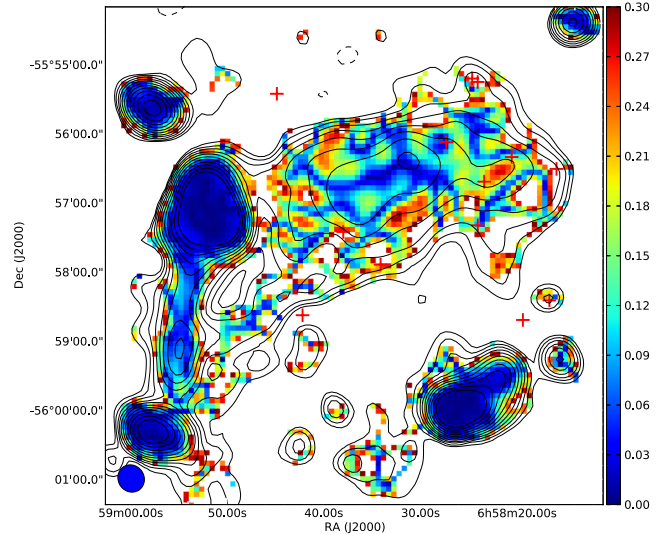
Figure 9. The spectral index error image for the 1.1–3.1 GHz spectral index map in Fig. 5 that was created using the wide-band method described in Section 3.4.1. The maximum spectral index error is 0.3. The contour levels are identical to those in Fig. 5.
